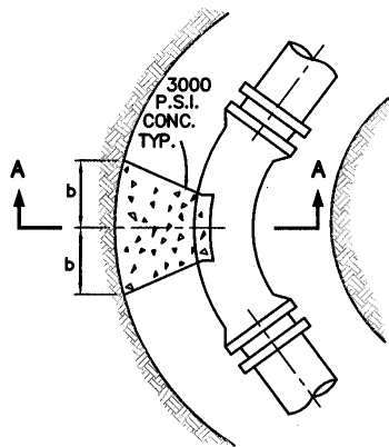
TYPICAL BEND PLAN
